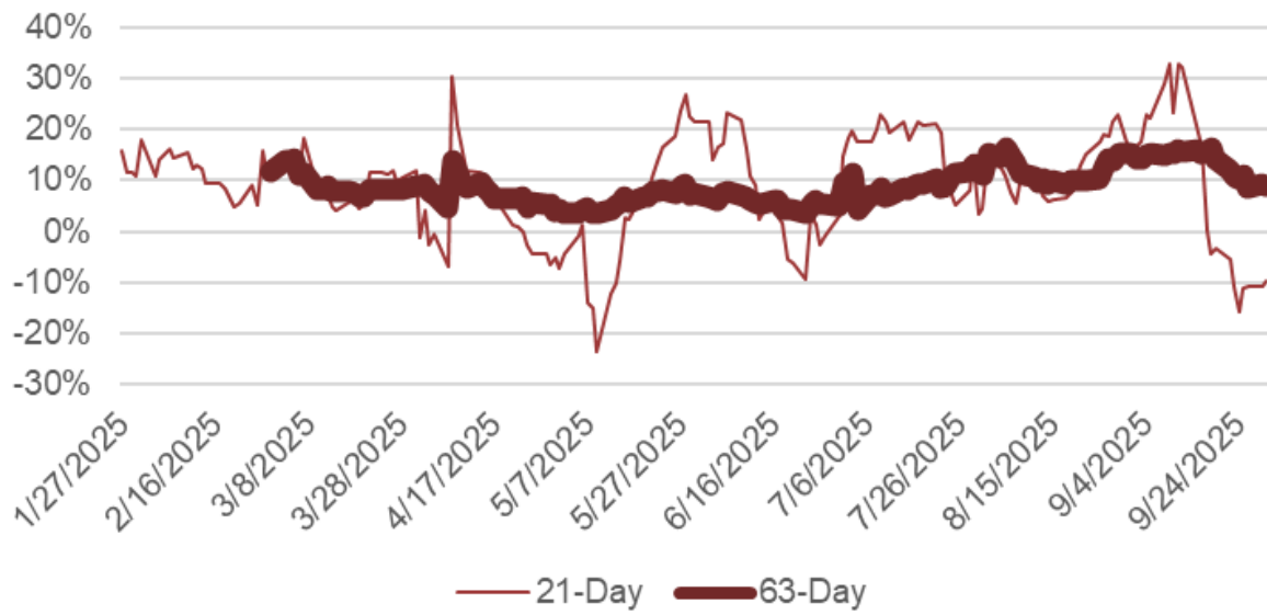
Rolling Cross-Correlation
